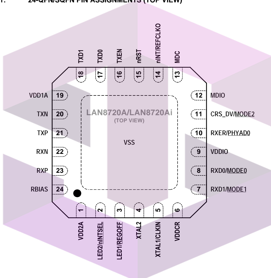
FIGURE 2-1: 24-QFN/SQFN PIN ASSIGNMENTS (TOP VIEW)
