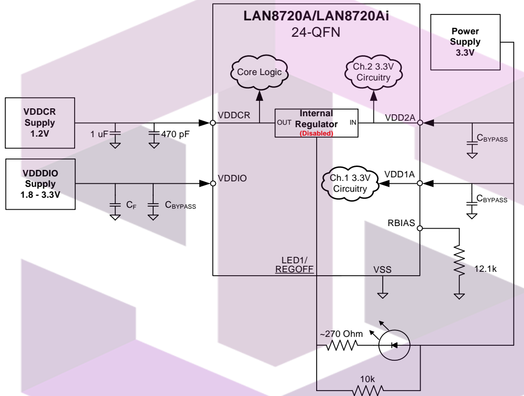
FIGURE 3-17: POWER SUPPLY DIAGRAM (1.2V SUPPLIED BY EXTERNAL SOURCE)
