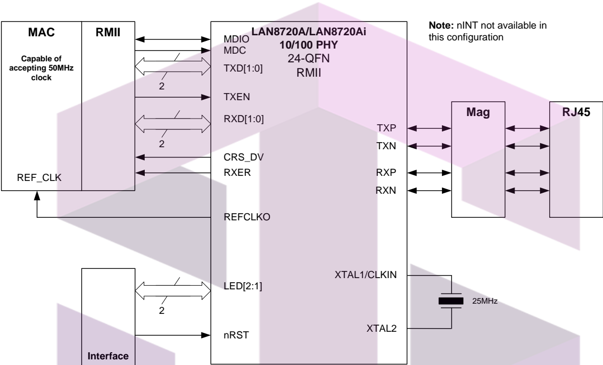
FIGURE 3-8: SOURCING REF_CLK FROM A 25MHZ CRYSTAL
