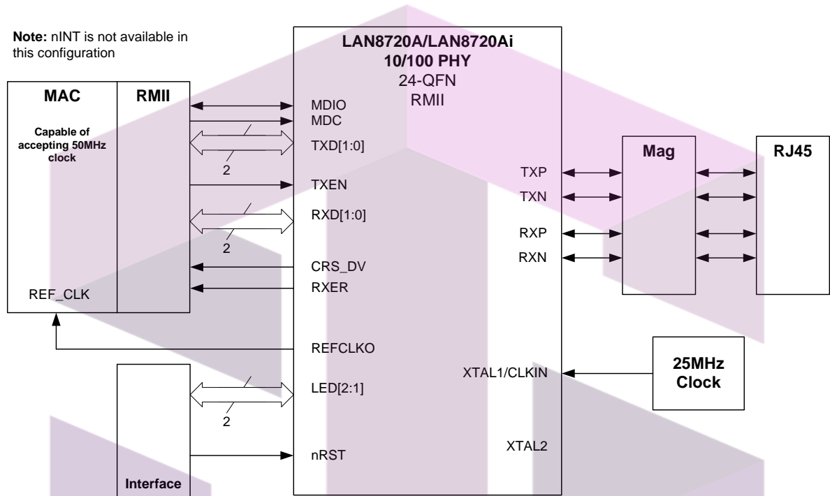
FIGURE 3-9: SOURCING REF_CLK FROM EXTERNAL 25MHZ SOURCE
